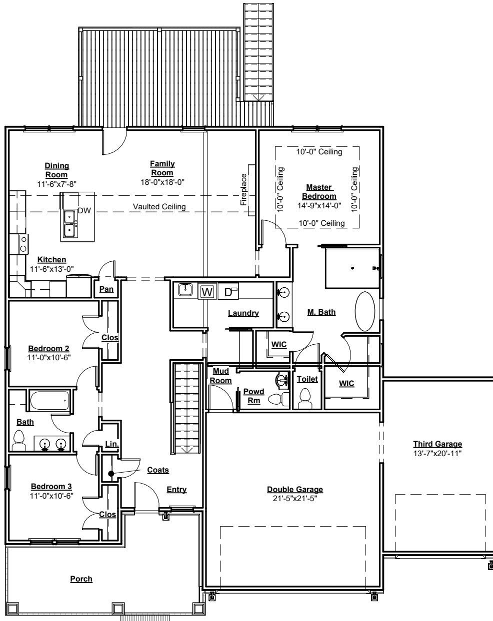
FIRST FLOOR
